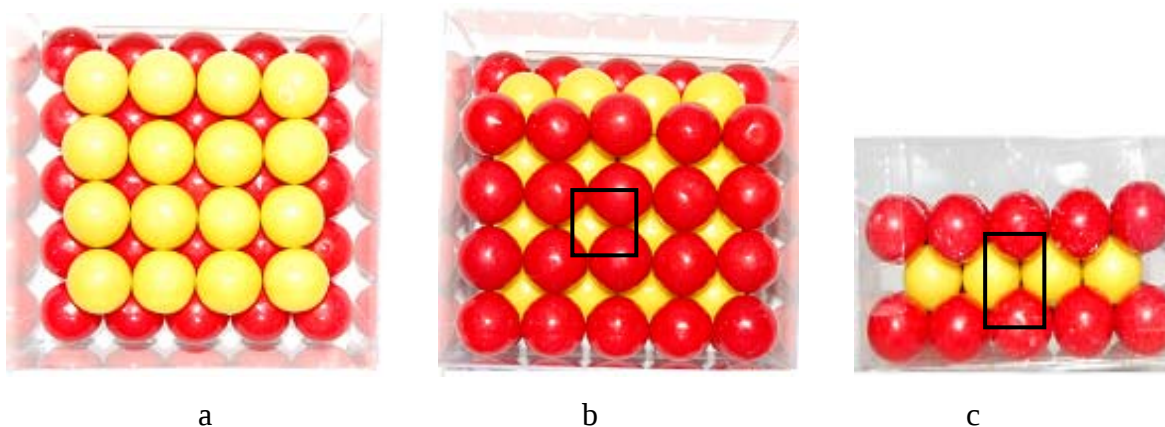
Figure 2. Body centred cube model. a) top view of the two layers, b) top view of three layers, c) side view of three layers.
