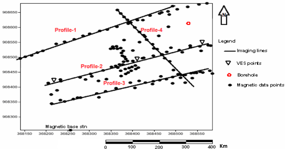
Figure 2. Electrical imaging survey traverses (solid lines), VES points (inverted triangles) and magnetic survey data points (solid dots). Only representative magnetic data points are shown to avoid congestion of the plot. Geographic coordinates in UTM.
