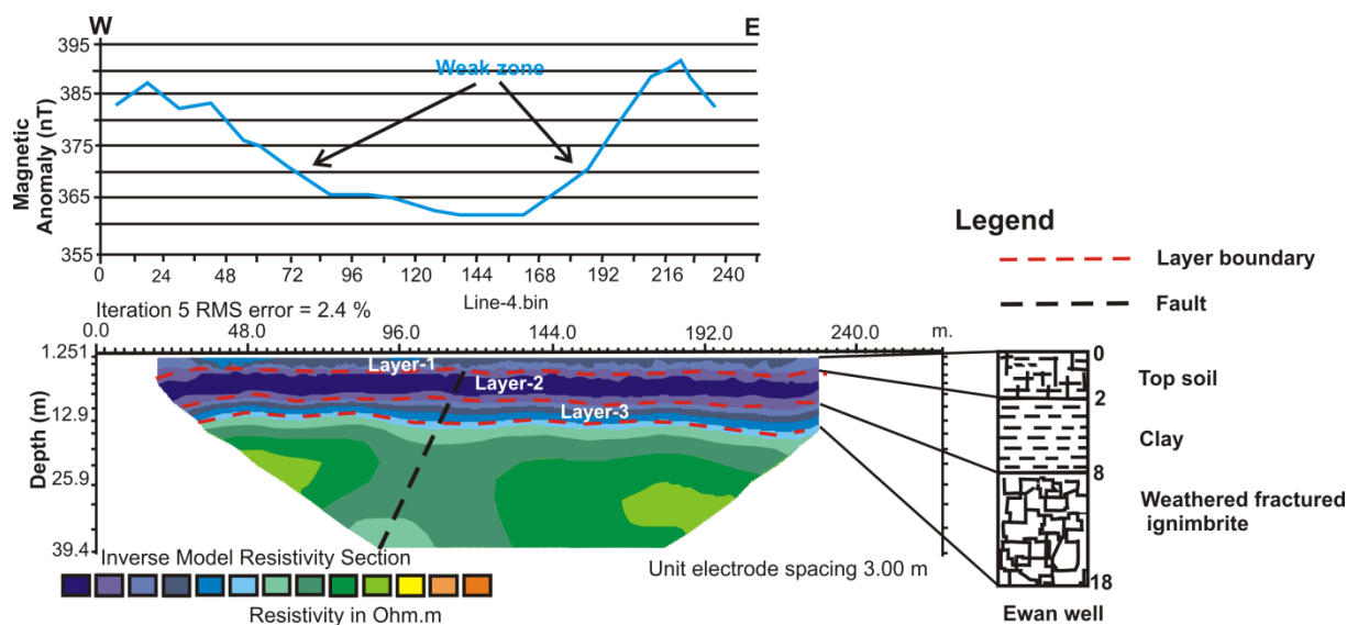
Figure 5. Combined interpretations of magnetic anomaly and 2D electrical resistivity imaging along Profile-4.
