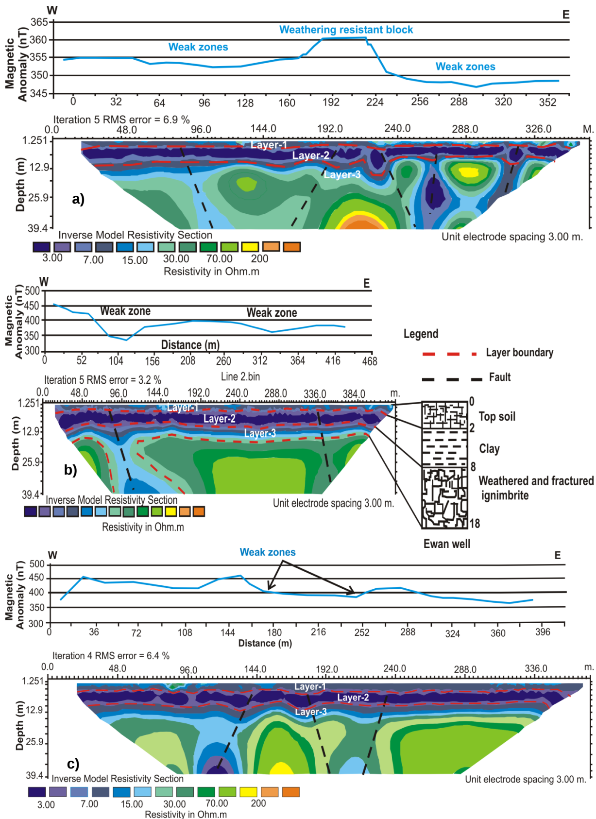
Figure 4. a, b, and c. Combined interpretations of magnetic anomaly and 2D electrical resistivity imaging inverse model sections for Profiles- 1, 2 and 3 respectively and correlation with lithologic log of the Ewan Well in (b) (Note the remarkable correlation between the magnetic profile plots and the resistivity model sections in depicting the weak zones).
