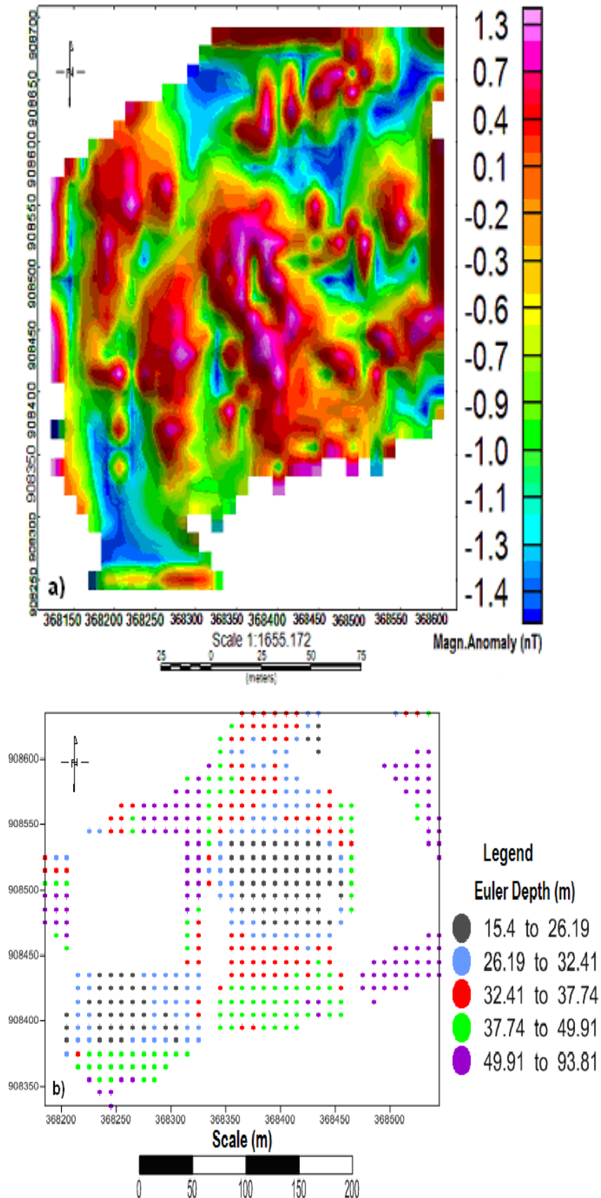
Figure 10(a). Tilt Derivative of Analytical Signal Map and (b) Euler Deconvolution depth map.
