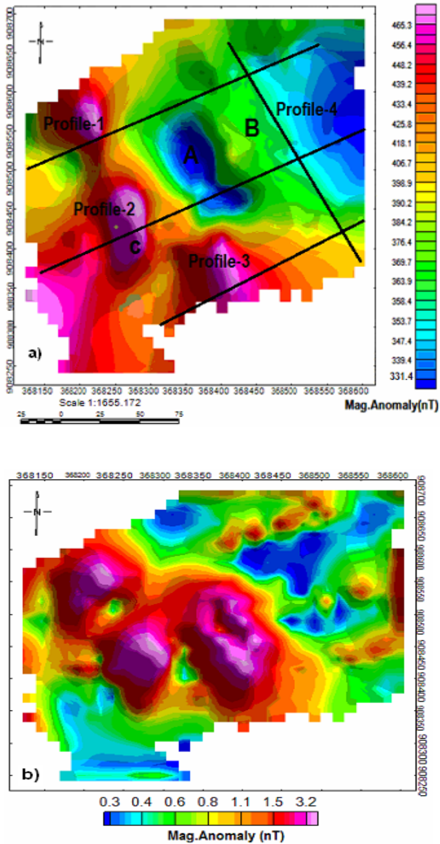
Figure 9. Magnetic Anomaly (a) and Analytical Signal Map (b).
