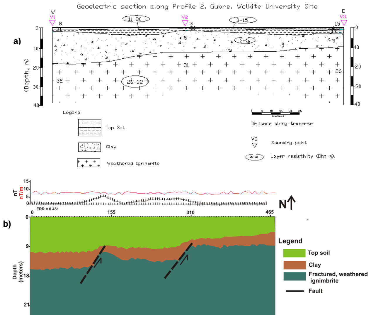
Figure 7. (a) Geoelectric section, and (b) Magnetic 2D model section along Profile-2.
