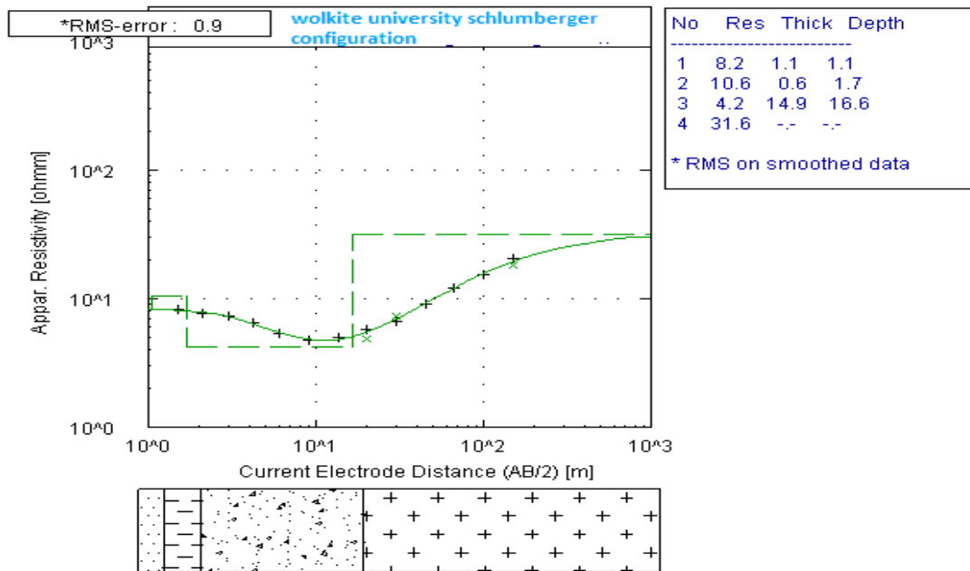
Figure 6. Typical 1D interpretation of VES (VES-1, Profile-2), and geological interpretation.
