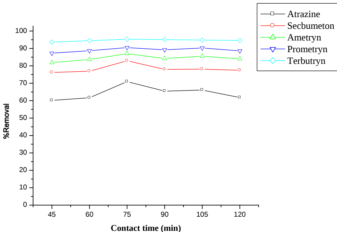
Figure 6. Effect of the contact time on the uptake of pesticide analytes. Experimental conditions: sample size, 25 mL; spiked concentration, 1 mg/L; agitation speed, 250 rpm; pH, 5; adsorbent dose, 0.7 g.
