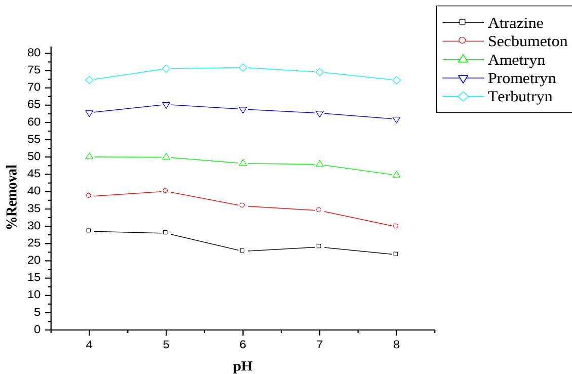
Figure 4. Effect of pH on the uptake of the pesticide analytes. Experimental conditions: sample size, 25 mL; spiked concentration, 1 mg/L; shaking speed, 100 rpm; contact time, 60 min; adsorbent dosage, 0.3 g.
