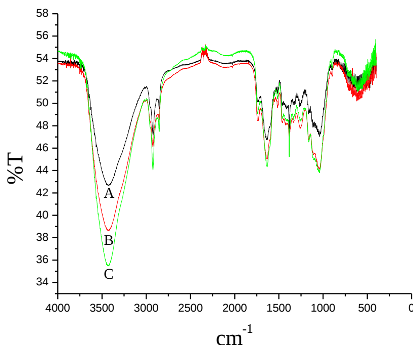
Figure 2. FT-IR spectra of the LBR in KBr disc; before treating with acid (A), after treating with acid (B) and pesticide loaded after treatment (C).
