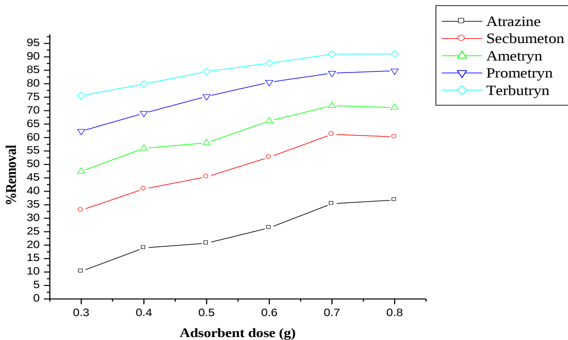
Figure 5. Effect of adsorbent dose on uptake of the pesticide analytes. Experimental conditions: sample size, 25 mL; spiked concentration, 1 mg/L; shaking speed, 100 rpm; contact time, 60 min; pH, 5.
