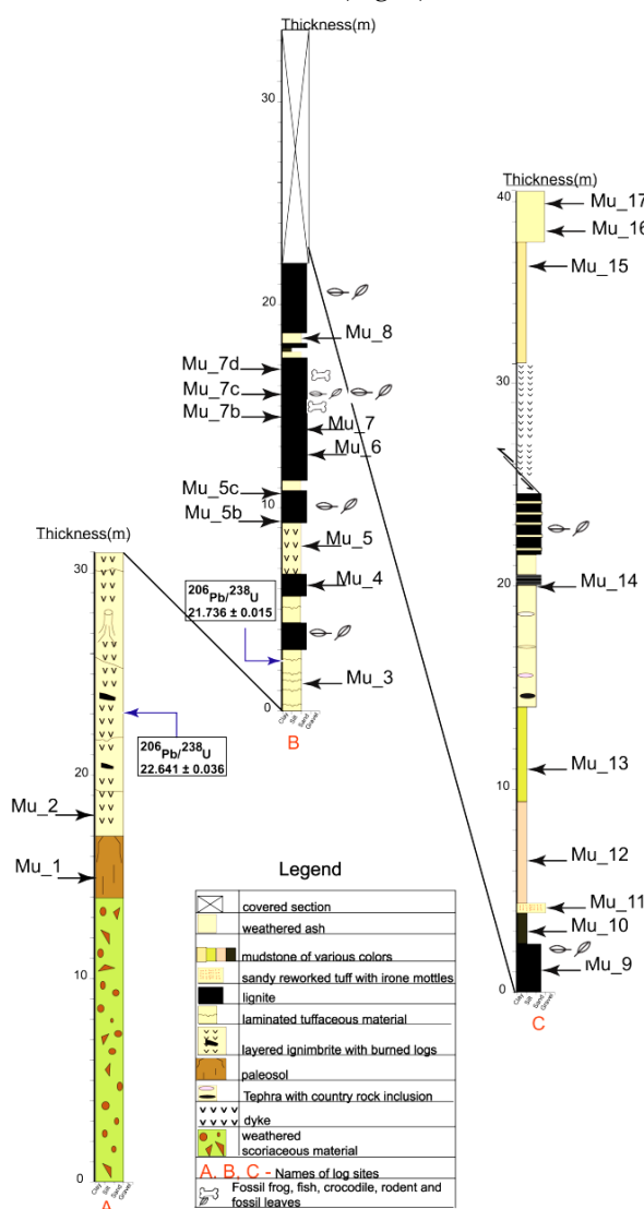
Figure 3. Stratigraphic section of the Mush basin sediments; labels of letters and numbers show locations of sample sites taken for radiometric, petrographic and XRD analyses.
