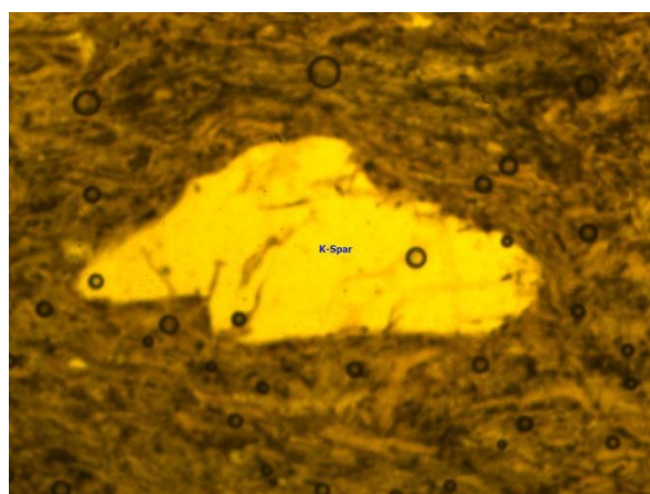
Photomicrograph of reworked ash (MU1) in plain polarized light, at 15 meters in stratigraphic Section_1 in Figure 3 (left). This photo shows abundant Potassium feldspar (K-spar) and reworked volcanic ash as groundmass. On the right side shows MU9 with organic matter as ground mass and few Potassium feldspar (sanidine) grains. MU9 is sampled at 1m in Section_3 of Figure 3.
