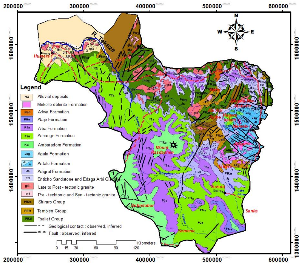
Figure 5. Simplified geological map of the TRB (Modified from EIGS, 1993).
