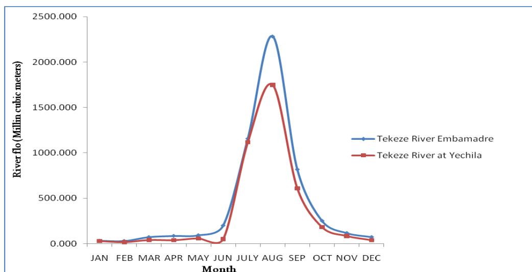
Figure 3. Hydrograph of the mean monthly river flow of Tekeze River.
