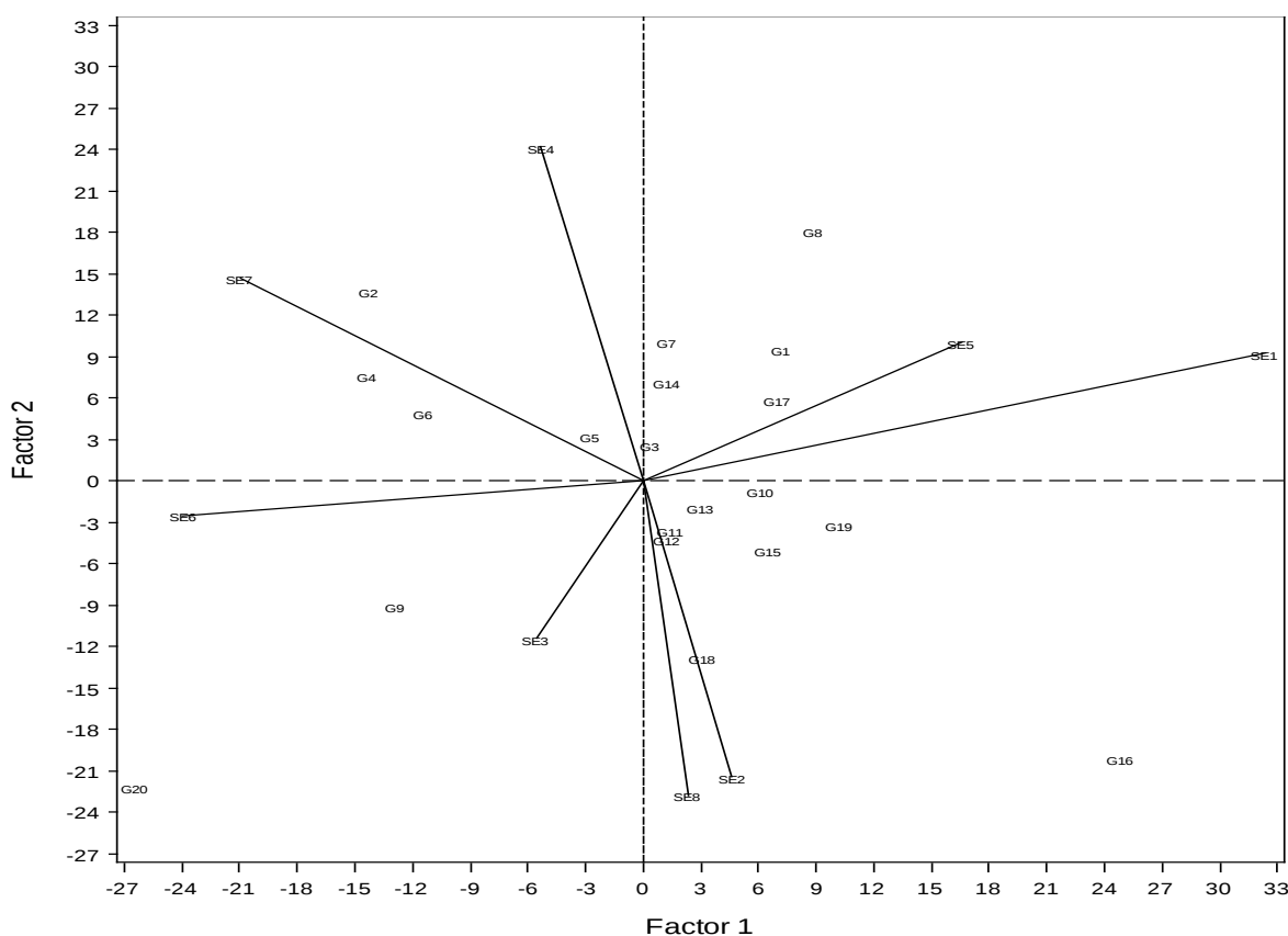
Figure 2. AMMI 2 biplot for grain yield of wheat genotypes showing the plotting of IPCA1 and IPCA2 of genotypes and environments with vectors. The angle and the projection of the vectors indicate the association among the environments.
