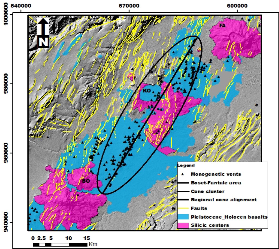
Figure 7. Boset-Fantale NE-SW regional vent alignment. Vents are restricted to Quaternary basaltic fields, their alignment being slightly oblique to the local fault trend.
