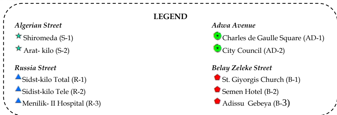
Fig. 2. Northern part of Addis Ababa containing 4 roads with 10 sampling sites.
