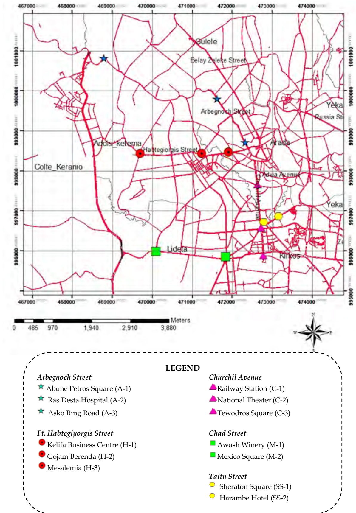
Fig. 3. Central part of Addis Ababa containing 5 roads with 13 sampling Sites.
