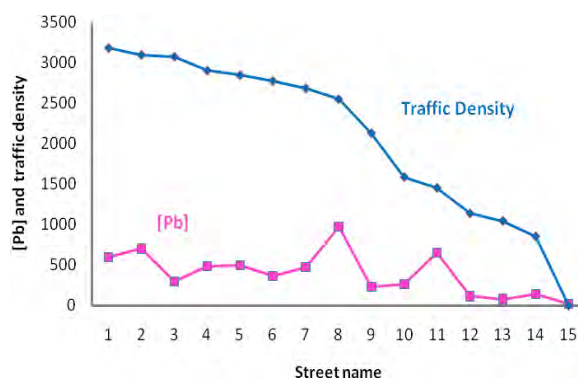
Fig. 6. Variation of lead concentrations with traffic densities. 1 (Alexander Pushkin Street), 2 (Zewditu Street), 3 (Debre Zeit Road ), 4 (Equatorial Guinea Street – Chad Street), 5 (Churchill Avenue), 6 (Taitu Street), 7 (Algerian Street – Africa Avenue), 8 (Adwa Avenue), 9 (Fit. H/Gyorgis Street), 10 (Dej. Belay Zeleke Street), 11 (Arbegnoch Street), 12 (Queen Elizabeth Street – Fikremariam Aba Techan Street), 13 (Akaki Main Road), 14 (Russia Street), 15 (Control).
