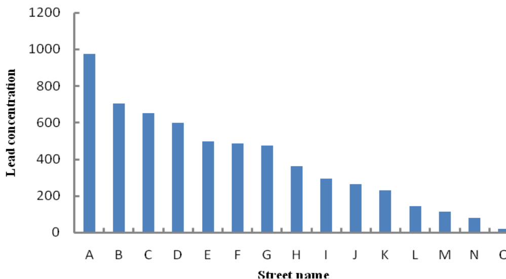
Fig. 5. Average concentrations of lead with respect to sampling streets in Addis Ababa city: A (Adwa Avenue), B (Zewditu Street), C (Arbengoch Street), D (Alexander Pushkin Street), E (Churchill Avenue), F (Equatorial Guinea Street – Chad Street), G (Algerian Street – Africa Avenue), H (Taitu Street), I (Debre Zeit Road), J (Dej. Belay Zeleke Street), K (Fit. H/Giyorgis Street), L (Russia Street), M (Queen Elizabeth Street – Fikremariam Aba Techan Street), N (Akaki Main Road) and O (Control), n = 3 .
