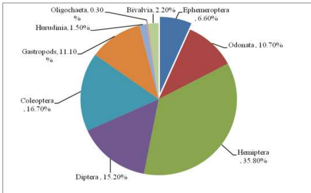
Figure 2. The percentage composition in classes of macro-invertebrates identified in Ketar River (Where, Oligochaeta for Oligochaeta).
