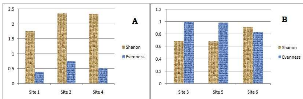
Figure 3. Diversity and evenness indices of macro-invertebrates among the sampling sites down the course of Ketar River.
