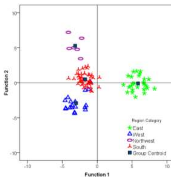
Figure 7: Scatter plot of the first two canonical discriminant function scores of green coffee beans at regional level based on CGA and Fatty acid composition
