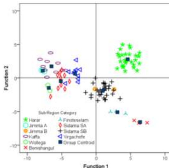
Figure 8. Scatter plot of the first two discriminant functions for green coffee beans by Sub-Region based on CGA contents
