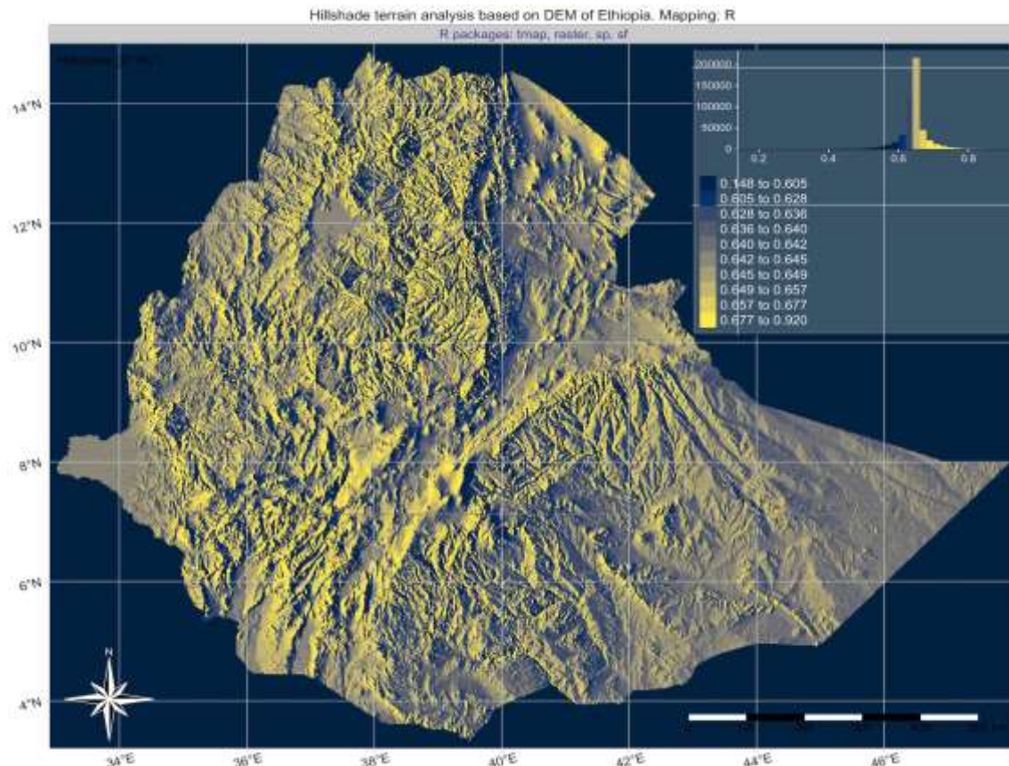
Figure 4. Hillshade relief map. Data: SRTM 90 DEM. Mapping: R. Source: author.
