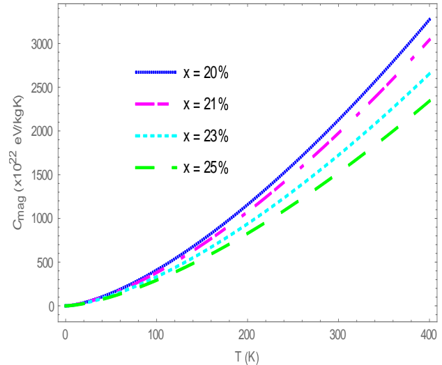
Figure 1. Magnon specific heat vs. temperature for different values of x when B = E = D = 0 .
