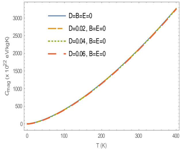
Figure 5. Magnon specific heat as a function of temperature for different values of D at the concentration x = 20\% with B and E set to zero.
