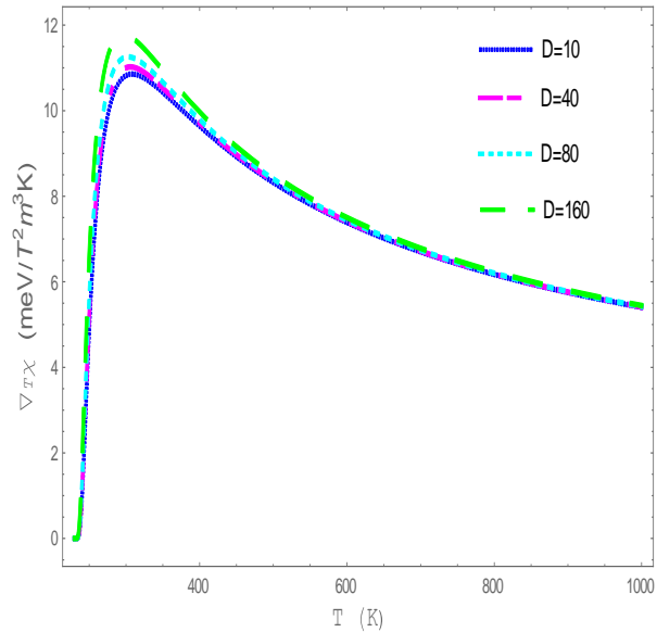
Figure 9. Temperature gradient of magnetic susceptibility vs. temperature for different values of D at x = 20\% , and E = B = 20 .
