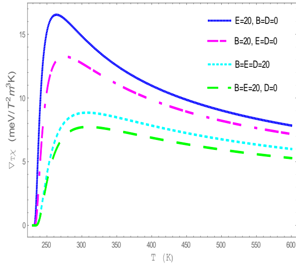
Figure 7. Temperature dependence of the magnetic susceptibility of GaFeSb for the same values of E , B , D and 20% magnetic impurity concentration.
