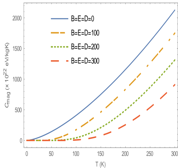
Figure 3. Magnon specific heat vs. temperature for varied similar values of B , E and D considered simultaneously at a concentration x = 20\% .
