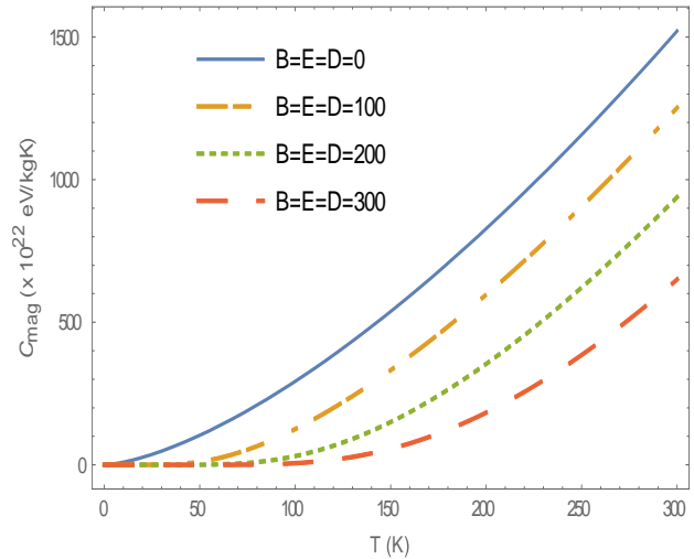
Figure 4. Magnon specific heat as a function of temperature with the same values of B ; E and D simultaneously at a concentration of x = 25\% .
