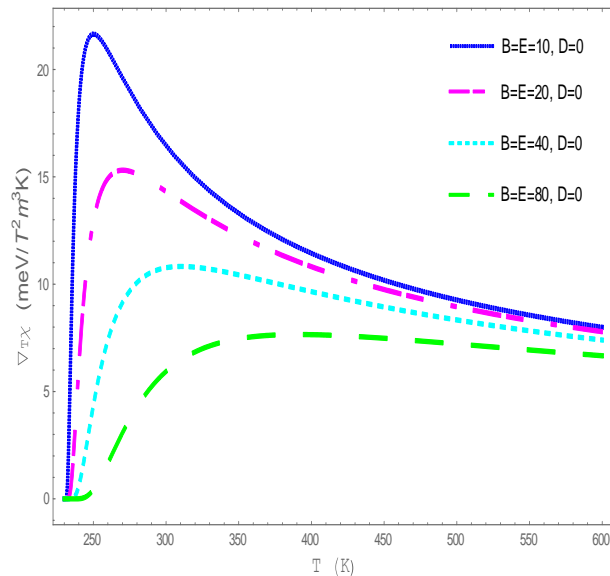
Figure 8. Temperature dependence of magnetic susceptibility with different values of B = E at a concentration of x = 20\% and D = 0 .
