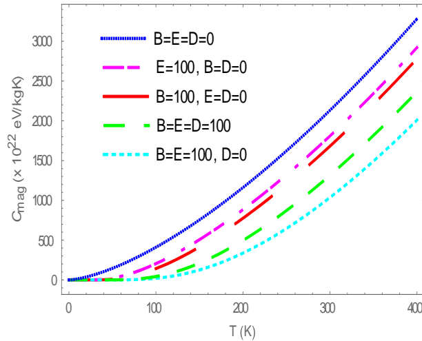
Figure 2. Magnon specific heat vs. temperature for the same values of B , E , and D , separately and all together, successively at 20% dopant concentration.
