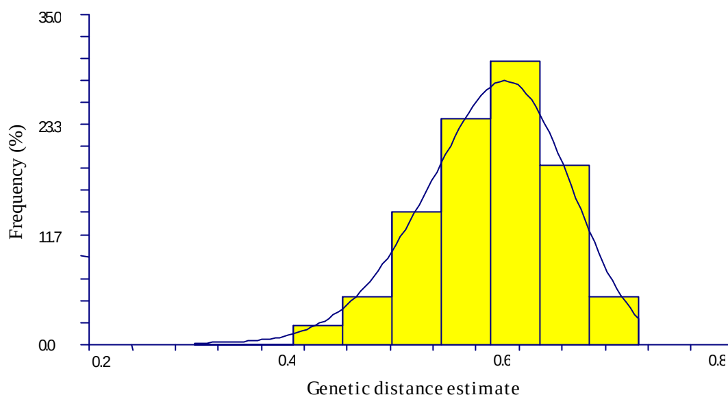
Fig. 2. Histogram depicting frequency distribution of genetic distances for all possible pairs of linseed accessions.
