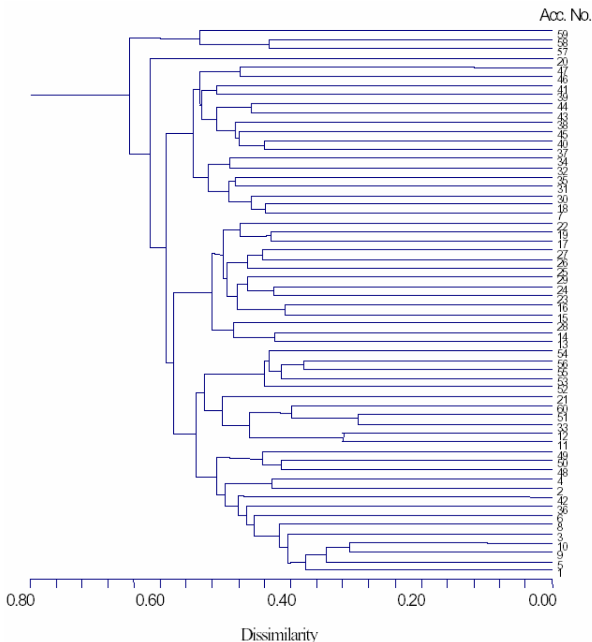
Fig. 1. Dendrogram indicating clusters of 60 accessions of linseed based on AFLP data, using UPGMA clustering method.
