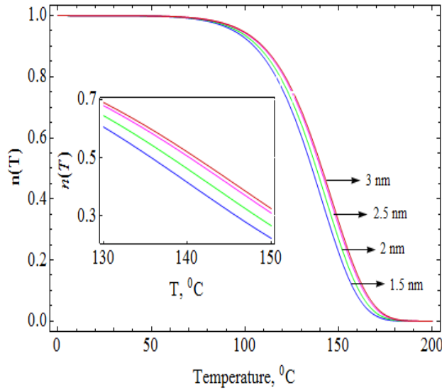
Figure 2: The normalized concentration of trapped electrons in the trap AT as a function of temperature for QDs of radii ranging between 1.5–3 nm. The values used for the simulation are: A_n = A_m = 10^{-9} \text{ cm}^3 \text{ s}^{-1} , N = M = 10^{16} \text{ cm}^{-3} , n_0 = m_0 = 2 \times 10^{14} \text{ cm}^{-3} , \beta = 1 \text{ K s}^{-1} , E = 0.75 \text{ eV} , and s = 10^8 \text{ s}^{-1} .
