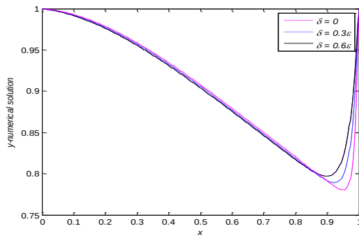
Fig. 1: The numerical solution of Example 1 with \varepsilon = 2^{-5} and N = 400 .
