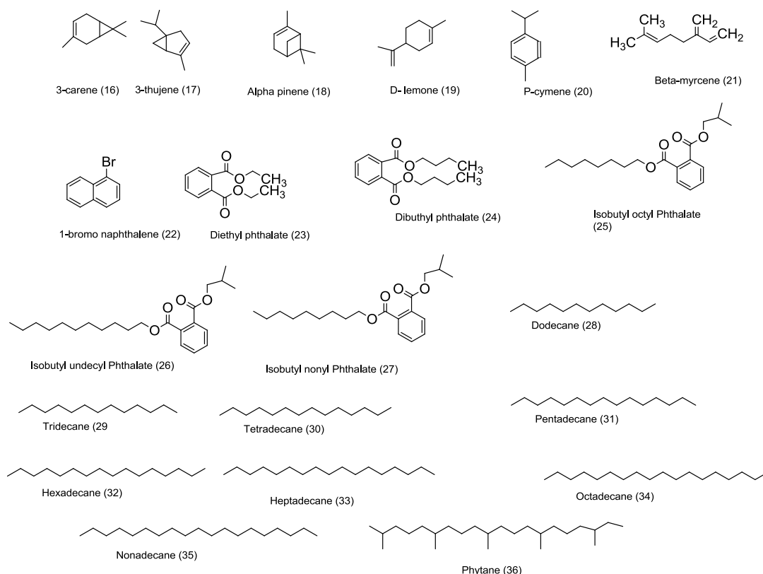
Figure 2: Structures of different detected additives and contaminants
