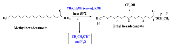
Scheme 1. Transesterification reaction of methyl hexadecanoate
