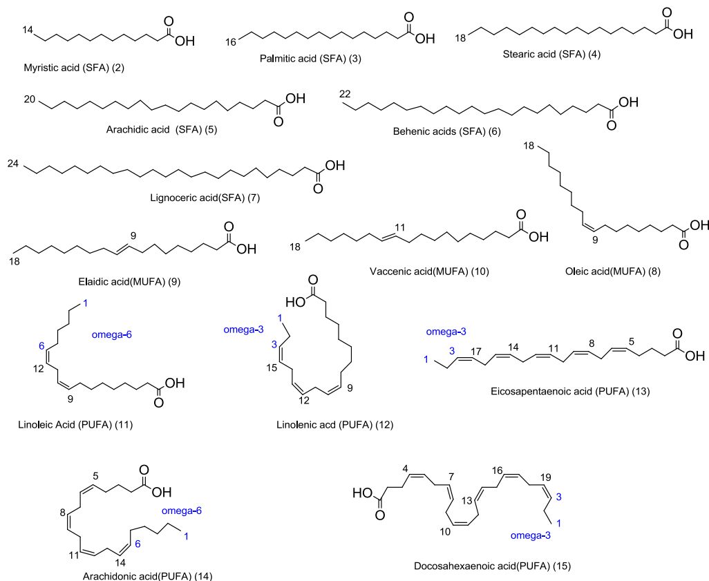
Figure. 1: Chemical structure of fatty acids, 2, 3, 4, 5, 6 and 7 are SFAs, 8, 9 and 10 are MUFAs and 11, 12, 13, 14 and 15 are PUFAs.
