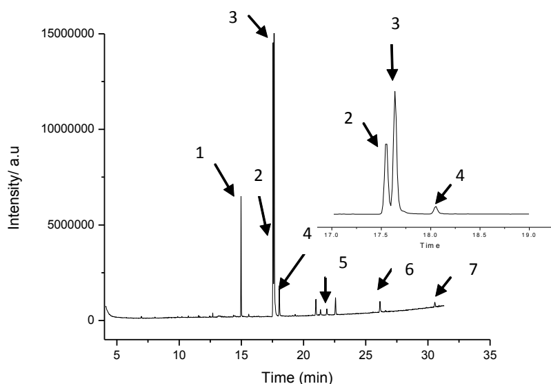
Figure 5. A representative chromatogram of edible oils: 1. Palmitic acid, 2. Stearic acid, 3. Oleic acid, 4. Linoleic acid, 5. Arachidic acid, 6. Behenic acid, 7. Lignoceric acid
