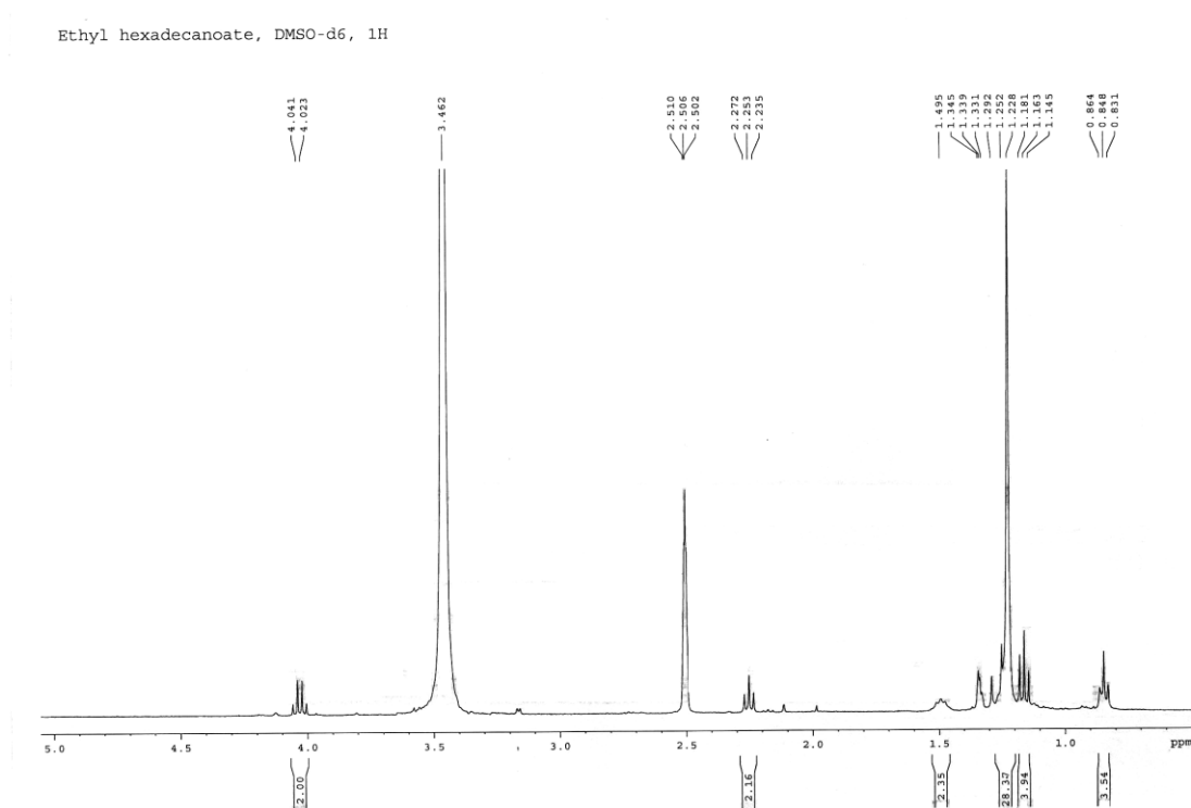
Figure 3. 1 H-NMR spectrum of Methyl hexadecanoate
