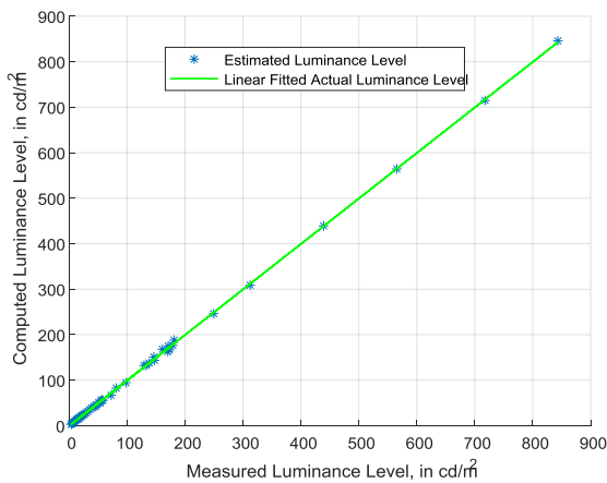
Figure 13 Validation for 0 – 900 \text{cd}/\text{m}^2 range
