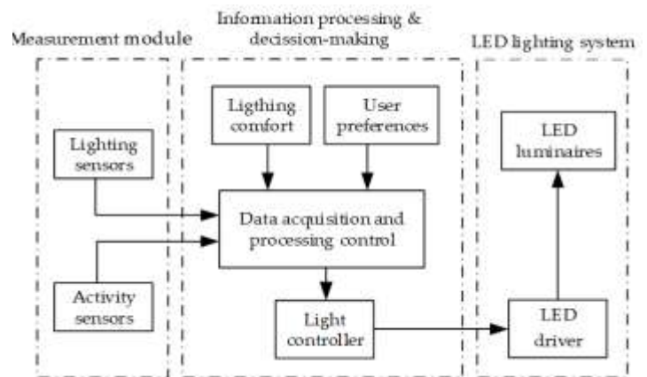
Figure 2 Typical smart luminaire system [14]
