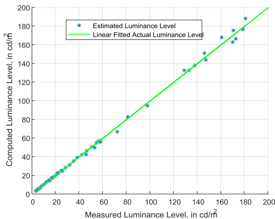
Figure 14 Validation for 0 – 200 \text{cd}/\text{m}^2 range
