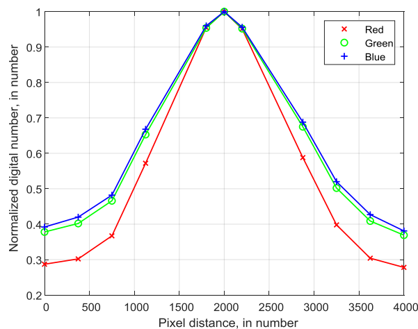
Figure 7 Red channel vignetting correction
