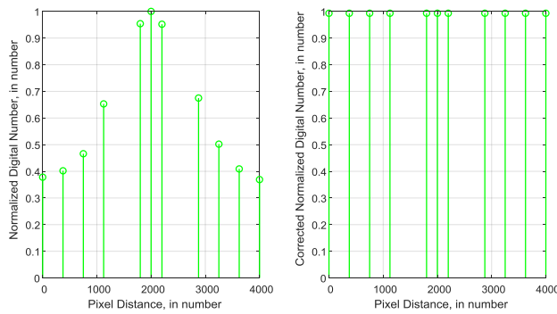
Figure 8 Green channel vignetting correction
