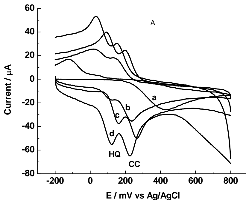
Fig. 3A. Cyclic voltammograms of 1 \times 10^{-3} \text{ mol L}^{-1} HQ and CC in PBS (pH 7.0) at different electrodes: bare GCE (a), poly(p-ASA)/GCE (b), MWCNTs/GCE (c) and poly(p-ASA)/MWCNTs/GCE (d). Scan rate: 20 \text{ mV s}^{-1} .
