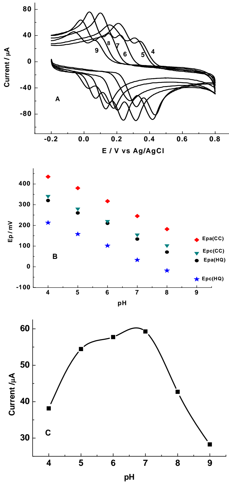
Fig. 5. (A) Cyclic voltammograms of poly(p-ASA)/MWCNTs/GCE in different pHs of 0.1 M PBS containing binary mixture of CC and HQ (each 1 \times 10^{-3} \text{ mol L}^{-1} ); (B) Plot of E_p vs pH of buffer solution; (C) The effect of pH of the solution on the anodic peak current of CC in a binary mixture of CC and HQ. pH range 4.0-9.0; scan rate: 0.1 \text{ Vs}^{-1} ; sensitivity: 100 \mu\text{A V}^{-1} .
