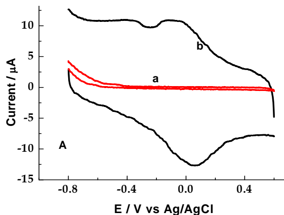
Fig. 2A. Cyclic voltammogram of bare GCE (a) and stabilized poly(p-ASA)/MWCNTs/GCE (b) in pH 7 PBS at a scan rate of 0.1 V s -1 .
