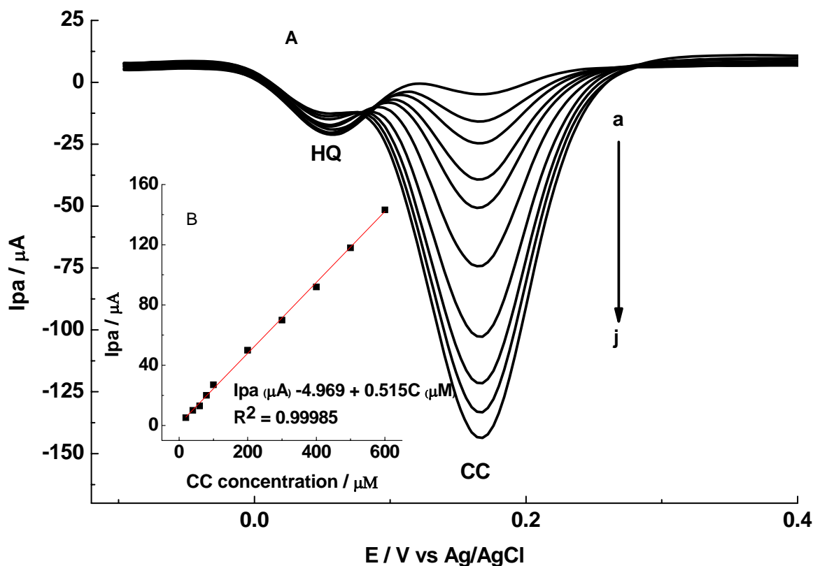
Fig. 7. (A) DPVs of poly(p-ASA)/MWCNTs/GCE in a binary mixture of variable concentration of CC and constant concentration of HQ in pH 7.0 PBS (a \rightarrow j: 20, 40, 60, 80, 100, 200, 300, 400, 500 and 600 \times 10^{-6} mol L -1 of CC and 1 \times 10^{-4} mol L -1 HQ); (B) plot of anodic peak current of CC at the modified GCE vs concentration. Scan rate: 50 mV s -1 ; pulse amplitude: 20 mV.
