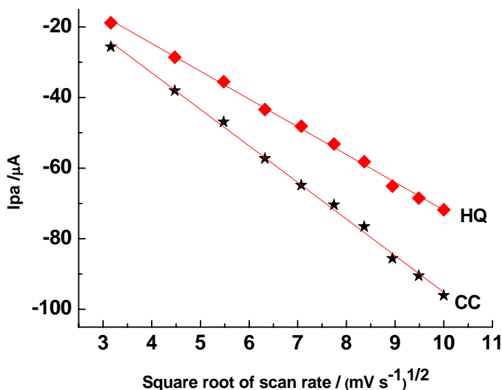
Fig. 4. Oxidative peak current vs square root of scan rate curve of 1 \times 10^{-3} mol L -1 CC and HQ in the range of 10 to 100 mV s -1 .
