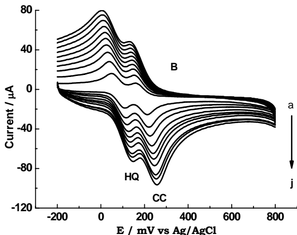
Fig. 3B Cyclic voltammograms of 1 \times 10^{-3} mol L -1 HQ and CC in pH 7.0 PBS at Poly(p-ASA)/MWCNTs/GCE at different scan rates (a → j: 10, 20, 30, 40, 50, 60, 70, 80, 90 and 100 mV s -1 ).
