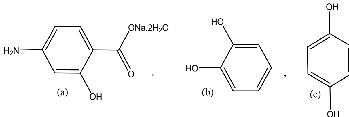
Scheme 1. Structural formula of dihydrated sodium salt of p -aminosalicylic acid ( p -ASA) (a), catechol (b) and hydroquinone (c).
