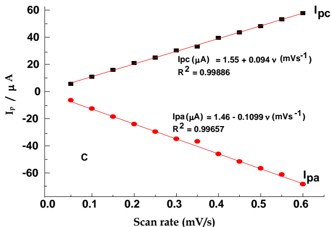
Fig. 2C. Plot of peak currents ( I_{pc} and I_{pa} ) vs scan rate ( v ).
