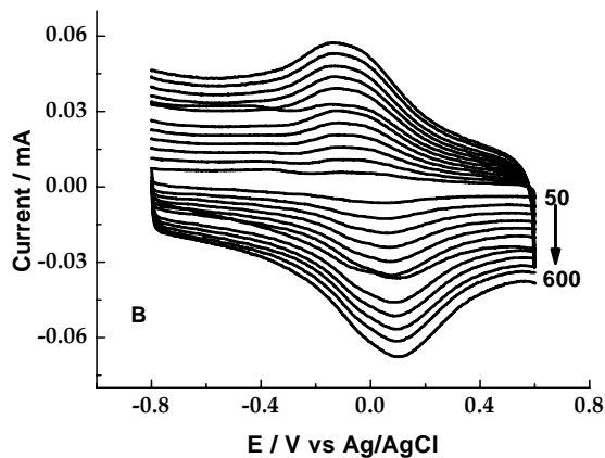
Fig. 2B. Cyclic voltammograms of poly(p-ASA)/MWCNTs/GCE in pH 7 PBS at different scan rates (from inner to outer waves: 50, 100, 150, 200, 250, 300, 350, 400, 450, 500, 550 and 600 \text{mV s}^{-1} ).
