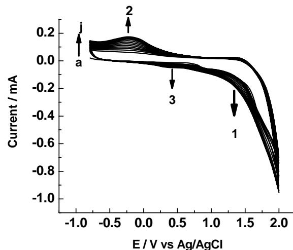
Fig. 1. Repetitive cyclic voltammograms (a-j) of 2.0 × 10 -3 mol L -1 para -aminosalicylic acid in 0.1M HNO 3 at the MWCNTs/GCE. Scan rate: 100 mV s -1 .
