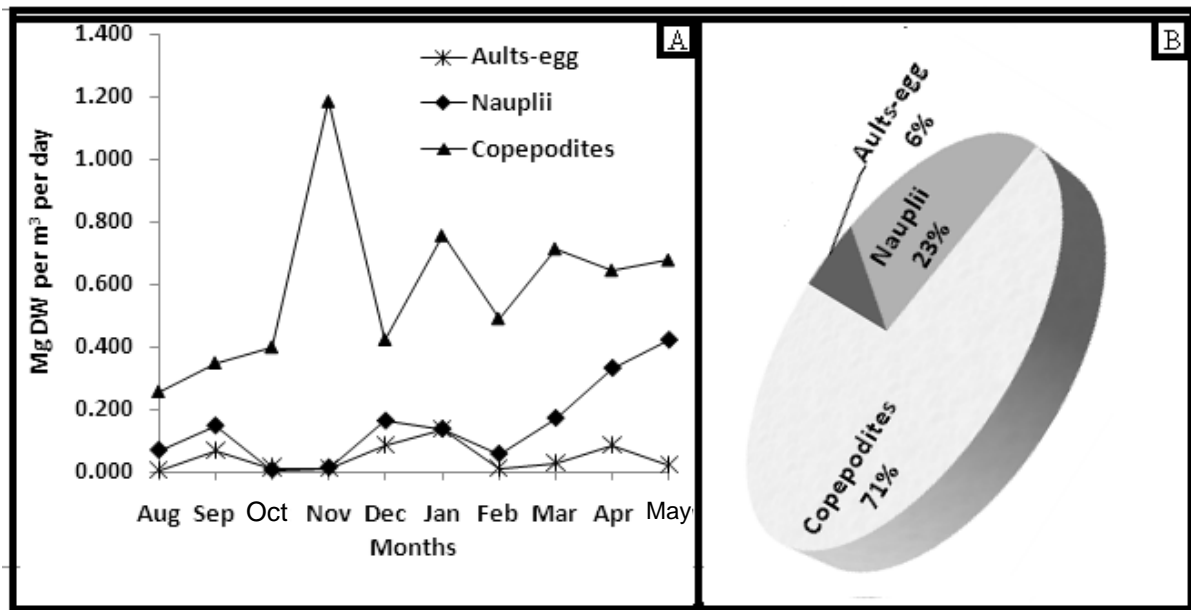
Fig. 3. Seasonal variation in production rates (mg DW m -3 ) (A) and percentage contribution (B) of nauplii, copepodites and adults-eggs of T. consimilis in Lake Kuriftu.
