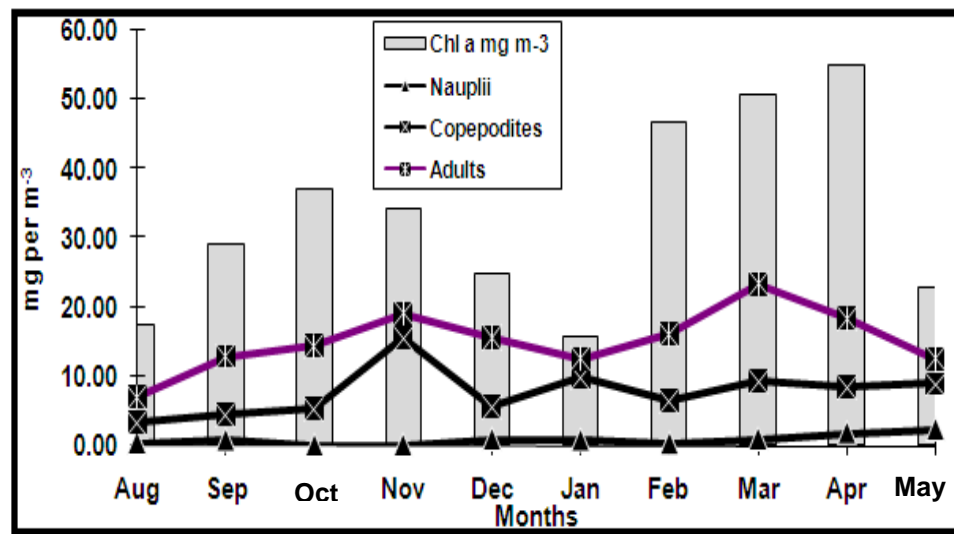
Fig. 2. Seasonal variation of biomass of nauplii, copepodites and adults of T. consimilis and phytoplankton biomass as chl a in Lake Kuriftu.
