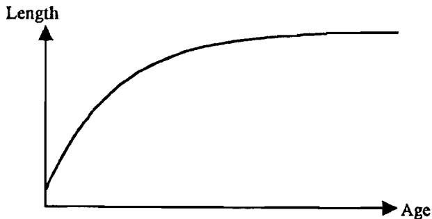
Fig. 3. General aspect of the von Bertalanffy Growth Curve.
