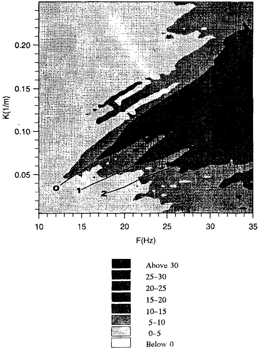
Fig. 2a. 2-D Amplitude spectrum of the data of Fig. 1a. (0, fundamental mode; 1, first higher mode; 2, second higher mode.)
