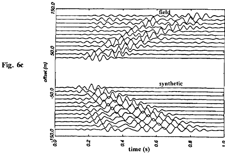
Fig. 6. Examples of synthetic and field data. Synthetic seismograms were computed using different Q values for near surface weathered structure: a) Q=5 , b) Q=50 , c) Q variable with depth between 5 at the free surface and 25 at 38 m of depth. Field are high cut-off filtered at the frequency of 30 Hz.
