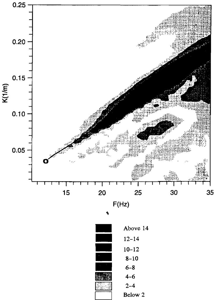
Fig. 2b. 2-D Amplitude spectrum of the data of Fig. 1b. (0, fundamental mode.)
