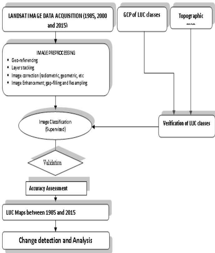
Figure 3. Schematic representations of LULC detection and analysis process (own work, 2013)
