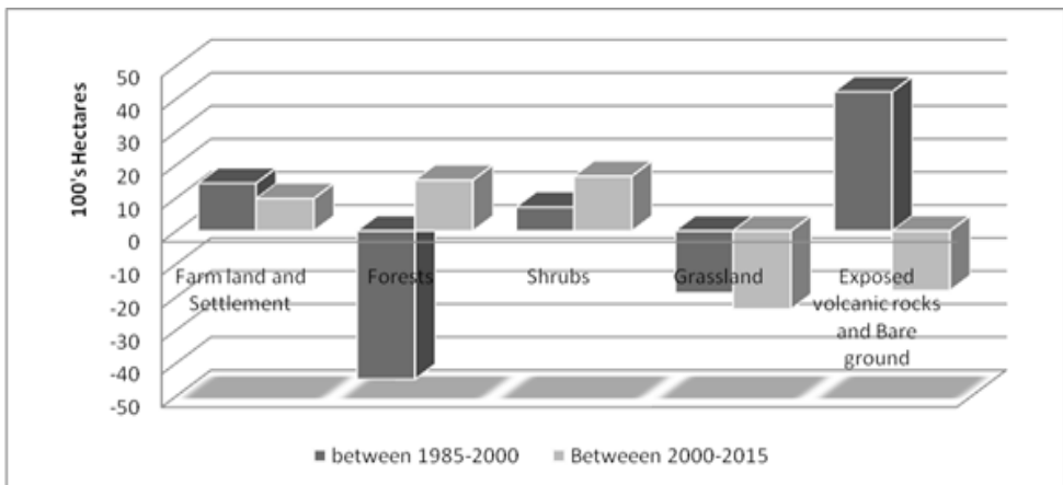
Figure 8: Graph showing the patterns of LULC change in the study area (1985 – 2015)
